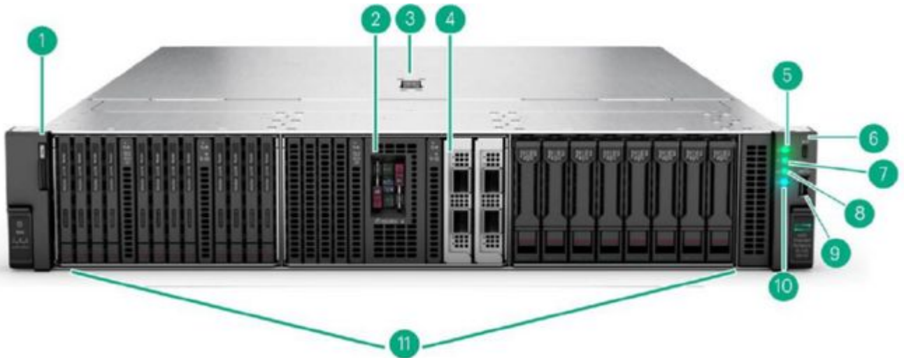
Front View - SFF/EDSFF CTO Server
